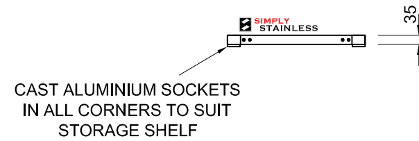
SIDE ELEVATION
