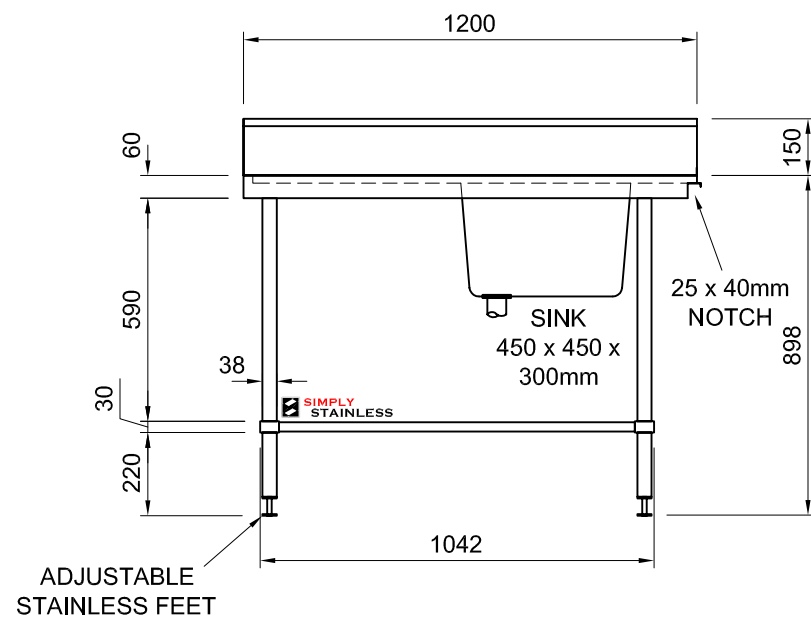
FRONT ELEVATION
