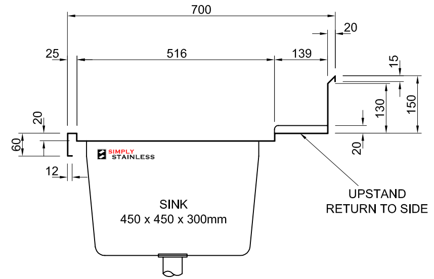
INLET BENCH PROFILE
