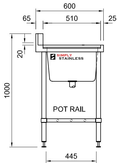
SIDE ELEVATION
