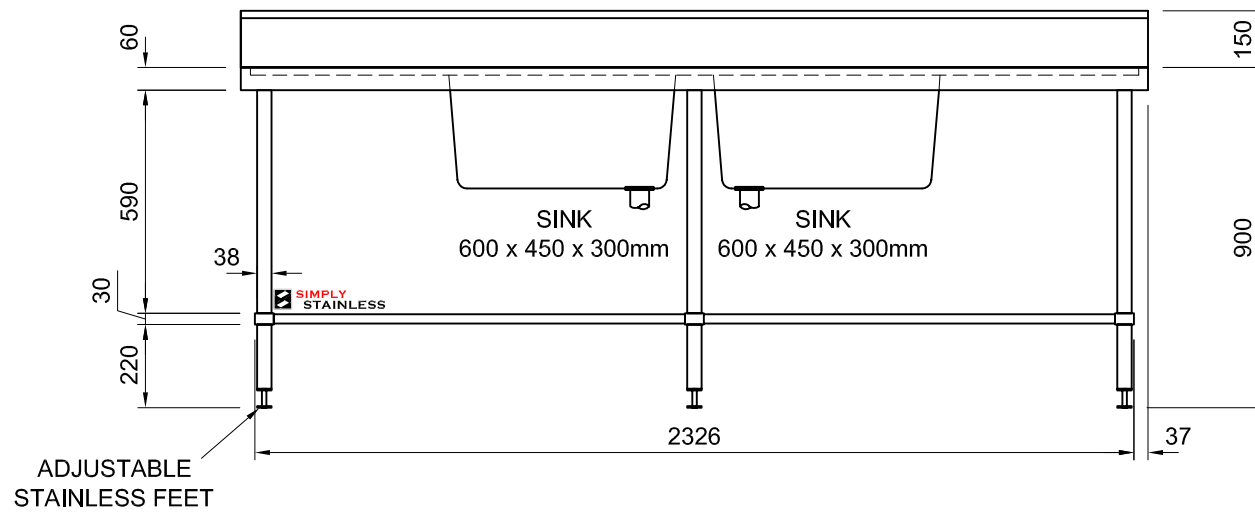
FRONT ELEVATION
